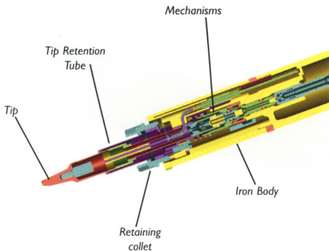
Cut-Away Drawing To show general principles or ProPiezo
